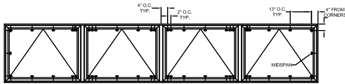
TYPICAL ELEVATION WITH FASTENER SPACING
