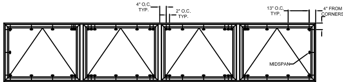
TYPICAL ELEVATION WITH FASTENER SPACING
