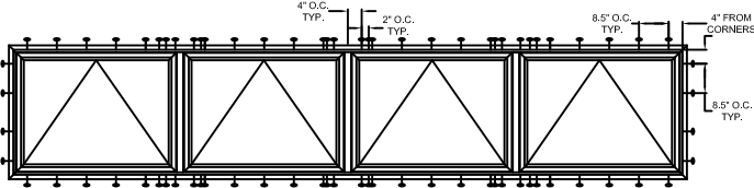
TYPICAL ELEVATION WITH FASTENER SPACING
