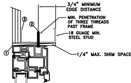
FRAME SECTION (TYP) VERTICAL SECTION
